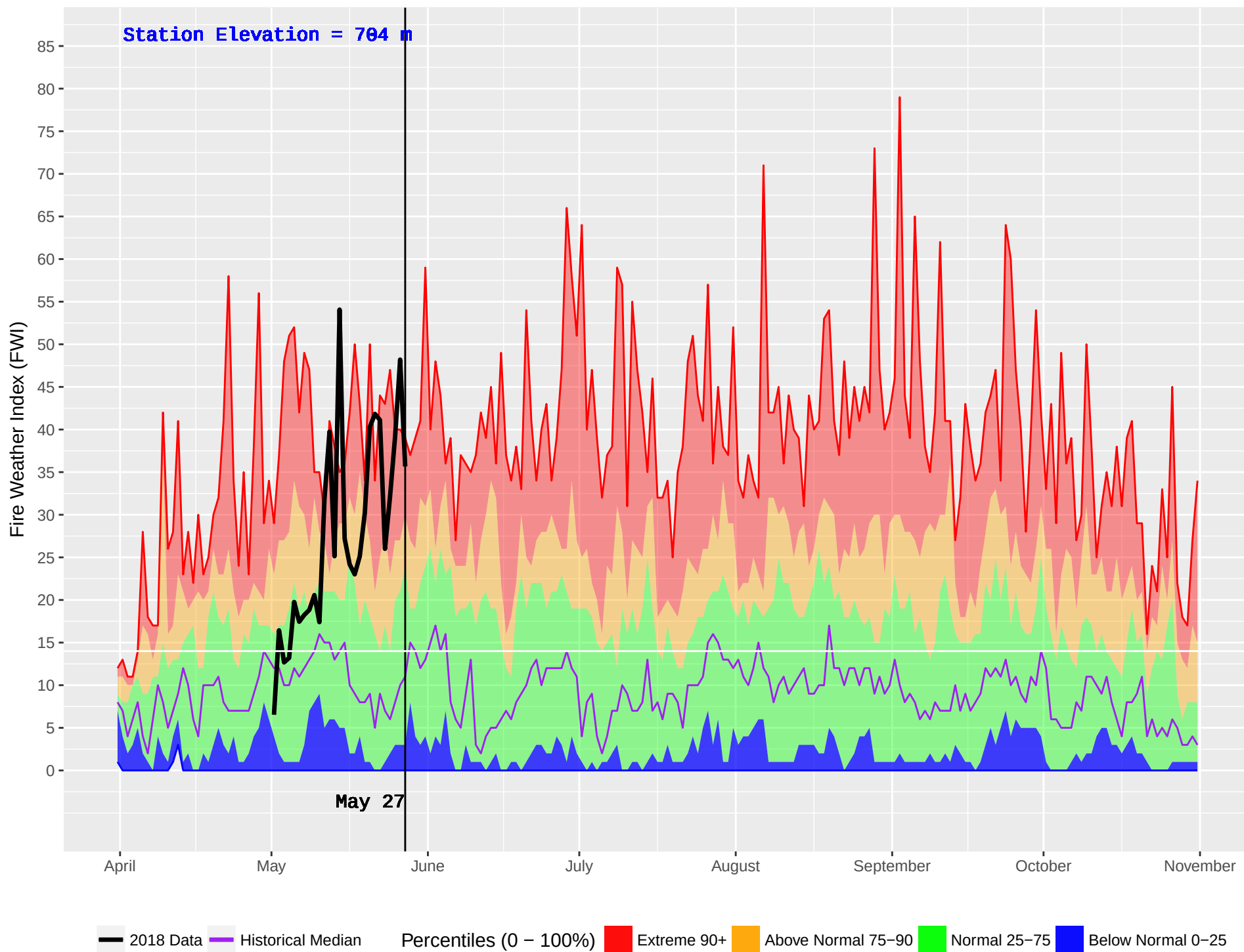
HUDSON HOPE (132) : Historical (1986–2016) and Current (2018) Noon Fire Weather Index (FWI)
