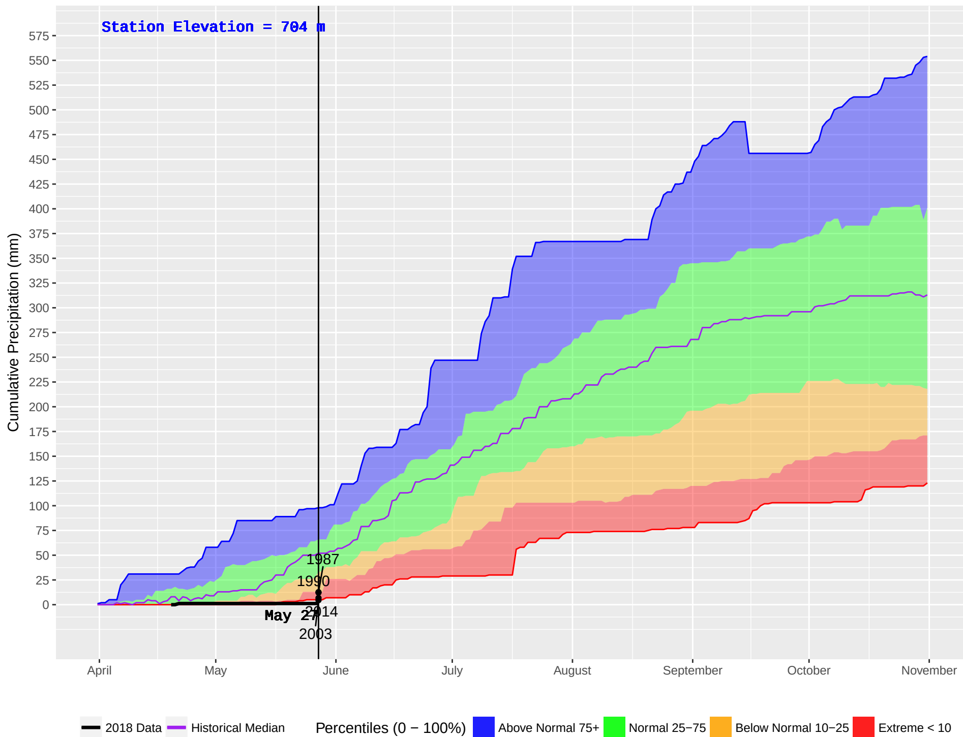
HUDSON HOPE (132) : Historical (1986–2016) and Current (2018) Noon Cumulative Precipitation
