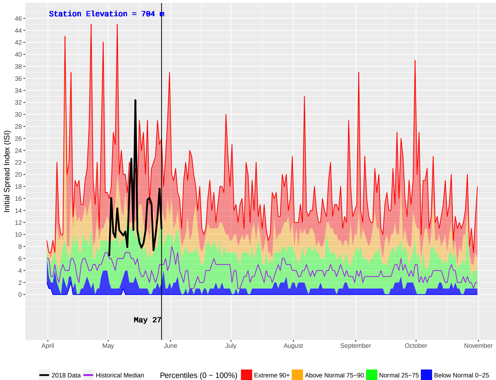
HUDSON HOPE (132) : Historical (1986–2016) and Current (2018) Noon Initial Spread Index (ISI)
