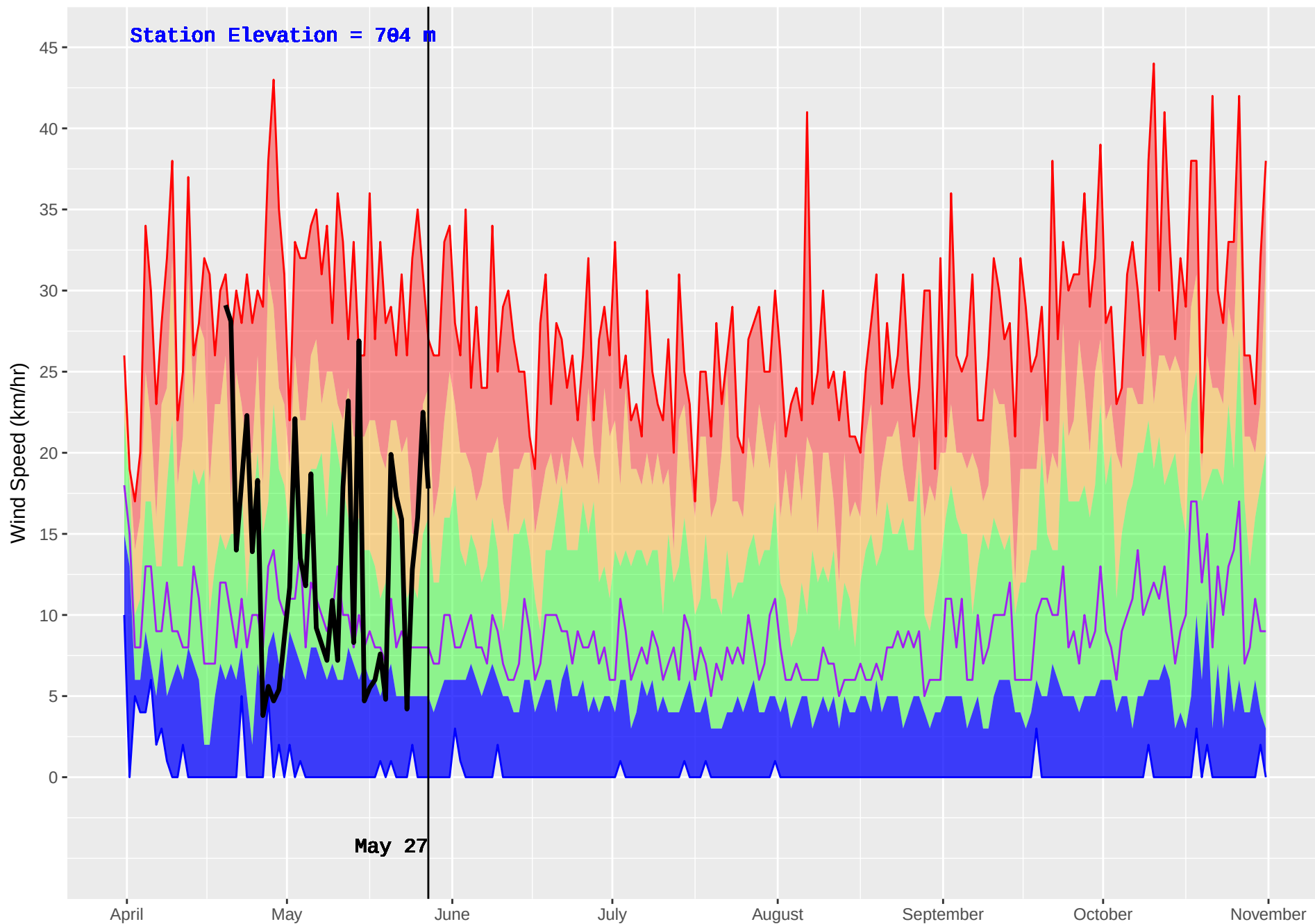
HUDSON HOPE (132) : Historical (1986–2016) and Current (2018) Noon Wind Speed
