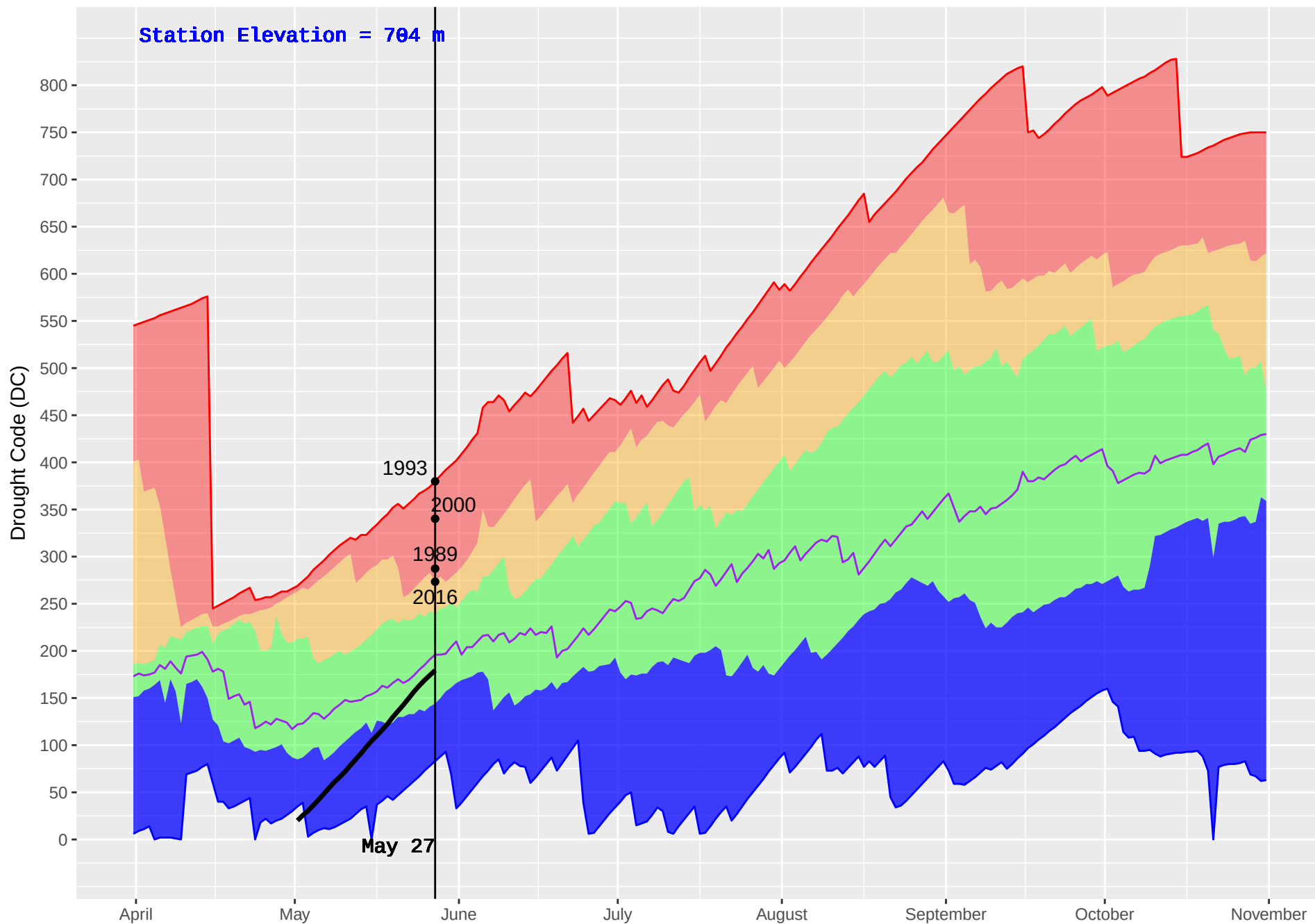
HUDSON HOPE (132) : Historical (1986–2016) and Current (2018) Noon Drought Code (DC)
